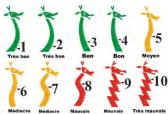
Figure 49 – Indices Atmo
